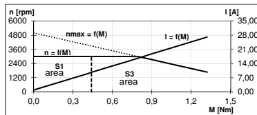
HSM7115-24-IG7.5, 24V, 3000rpm
