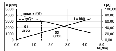
HSM7145-24-IG7.5, 24V, 3000rpm
