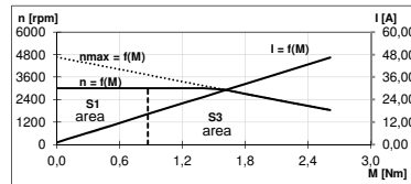
HSM7130-24-IG7.5, 24V, 3000rpm
